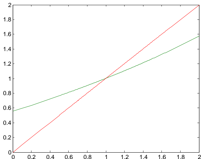
Figure 6: Optimal structured product for an CARA-investor with \alpha = 0.5 .
